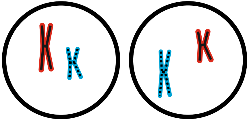
Prophase 2
