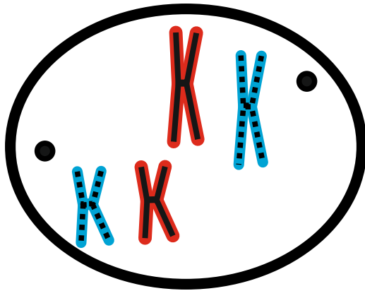
Prophase 1
