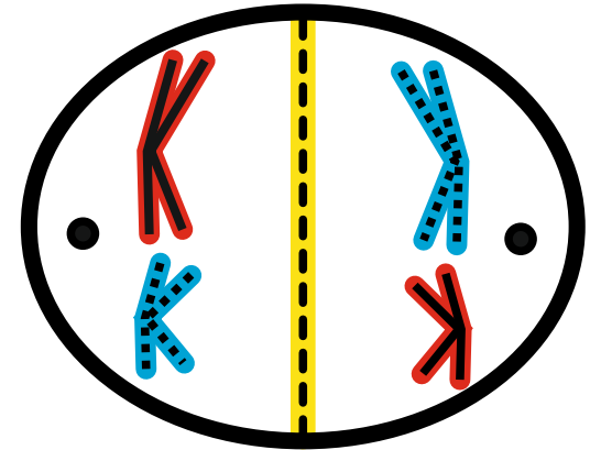
Anaphase 1
