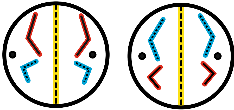
Anaphase 2
